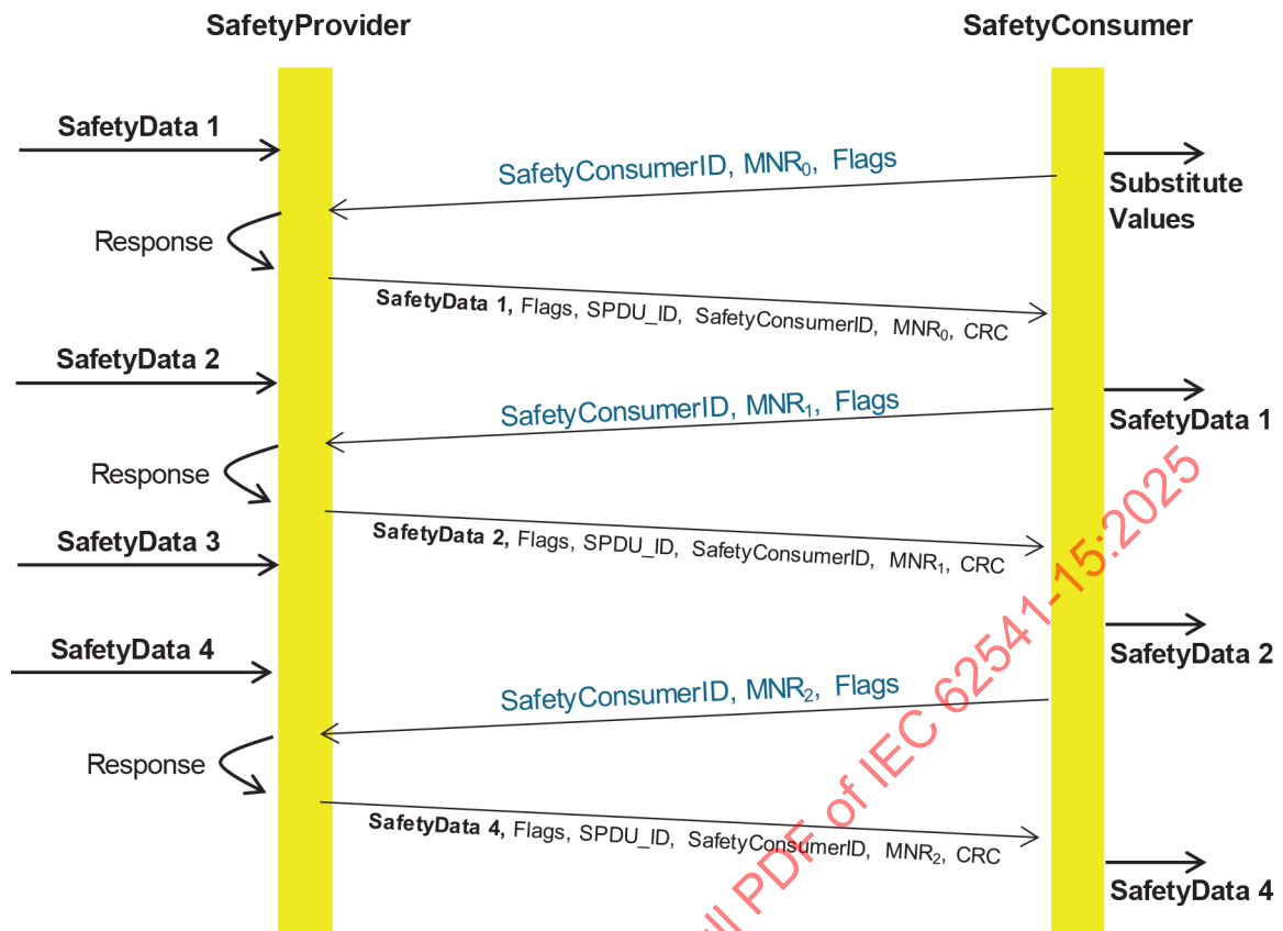
Figure 13 – Sequence diagram for requests and responses (Client/Server)
