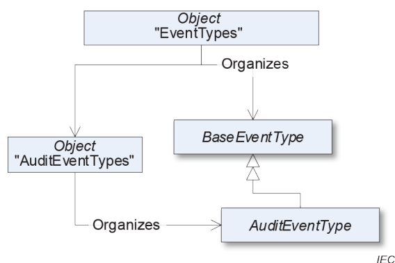
Figure 7 – EventTypes organization
