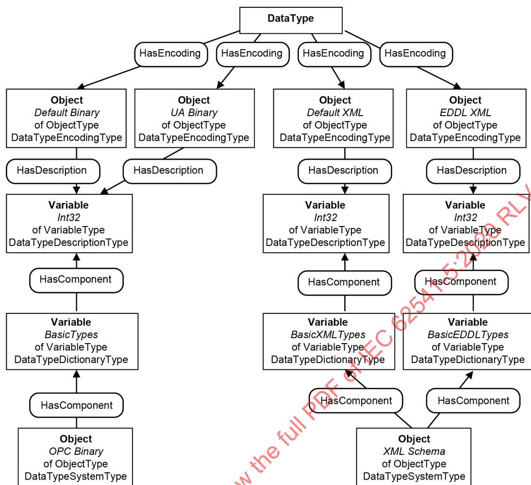
Figure D.2 – Example of DataType modelling
