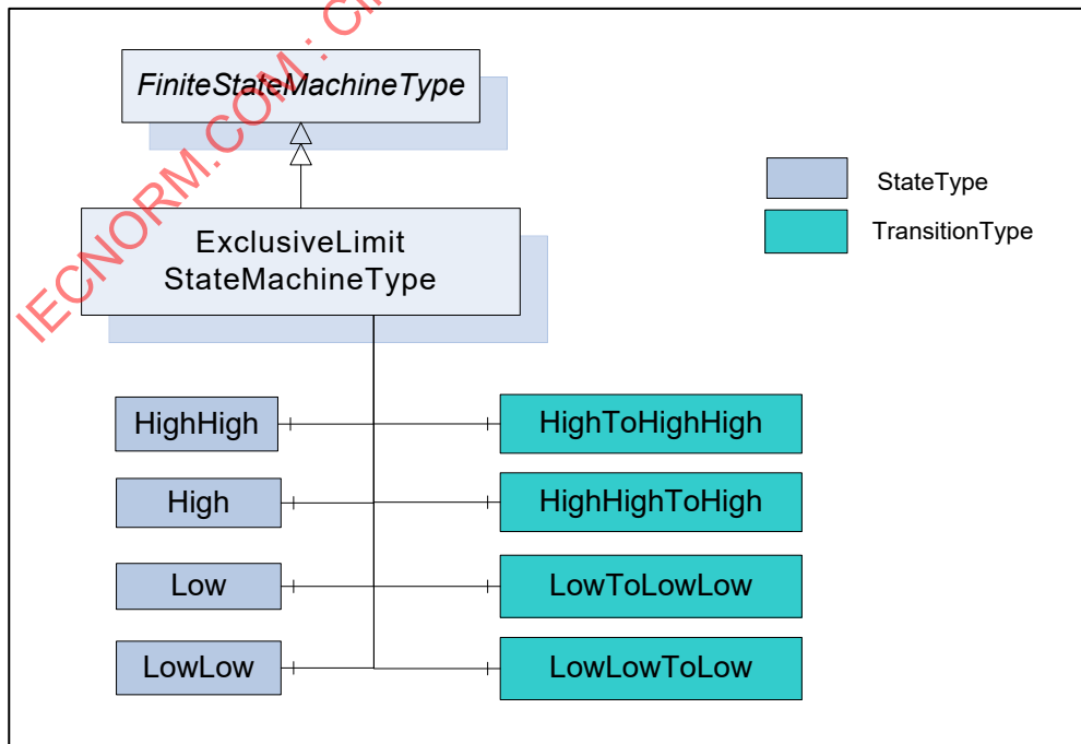
Figure 17 – ExclusiveLimitStateMachineType
