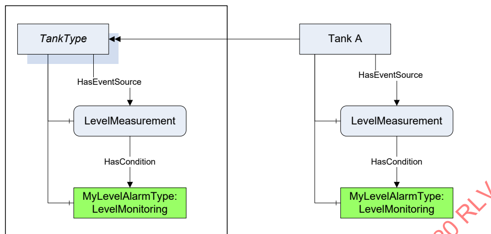
Figure 26 – Use of HasCondition in an InstanceDeclaration
