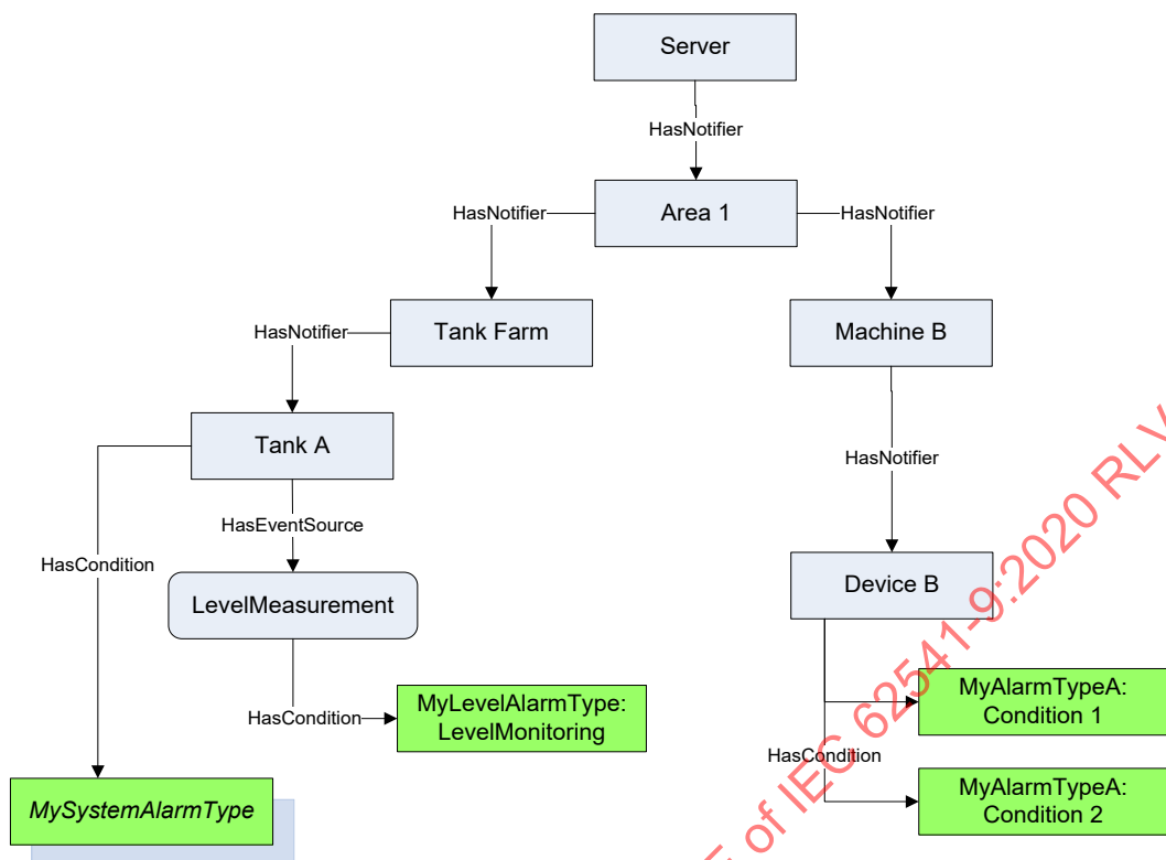
Figure 25 – Use of HasCondition in a HasNotifier hierarchy
