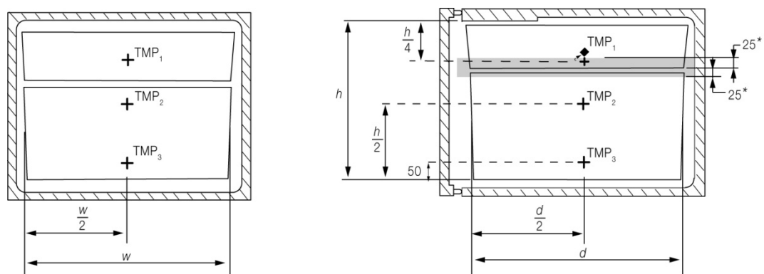
(a) Sensor TMP1 relocated to maintain clearance to drawer liner (unfrozen)
