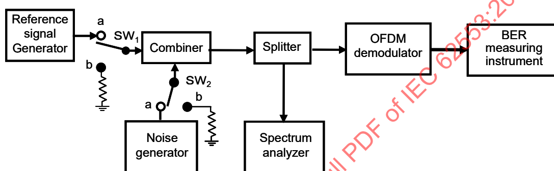
Figure B.5 – Inherent degradation of OFDM demodulator measurement system
