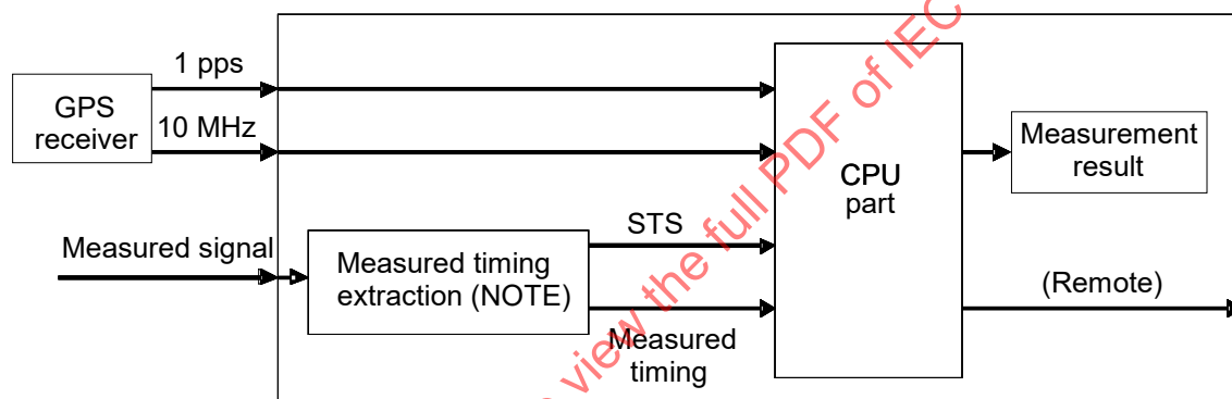
Figure A.10 – General measurement system for cases 7, 8 and 15,16
