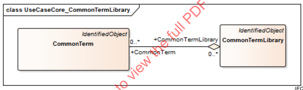
Figure 15 – Class diagram UseCaseCoreConcepts::UseCaseCore_CommonTermLibrary
