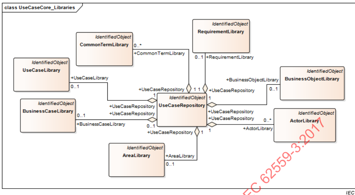
Figure 8 – Class diagram UseCaseCoreConcepts::UseCaseCore_Libraries
