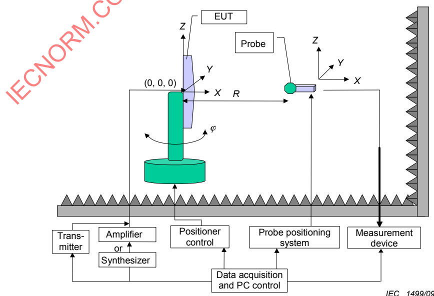
Figure A.1 – Block diagram of the EUT measurement system
