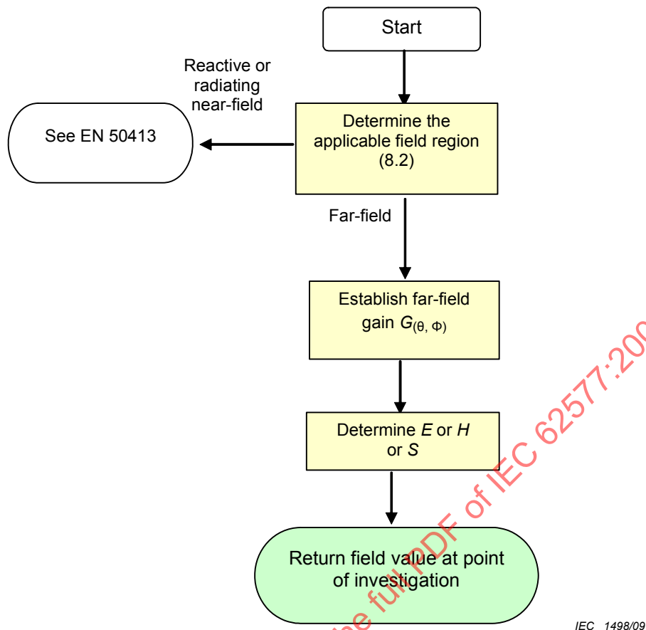
Figure 1 – Alternative routes to calculate E -field, H -field values at point of investigation
