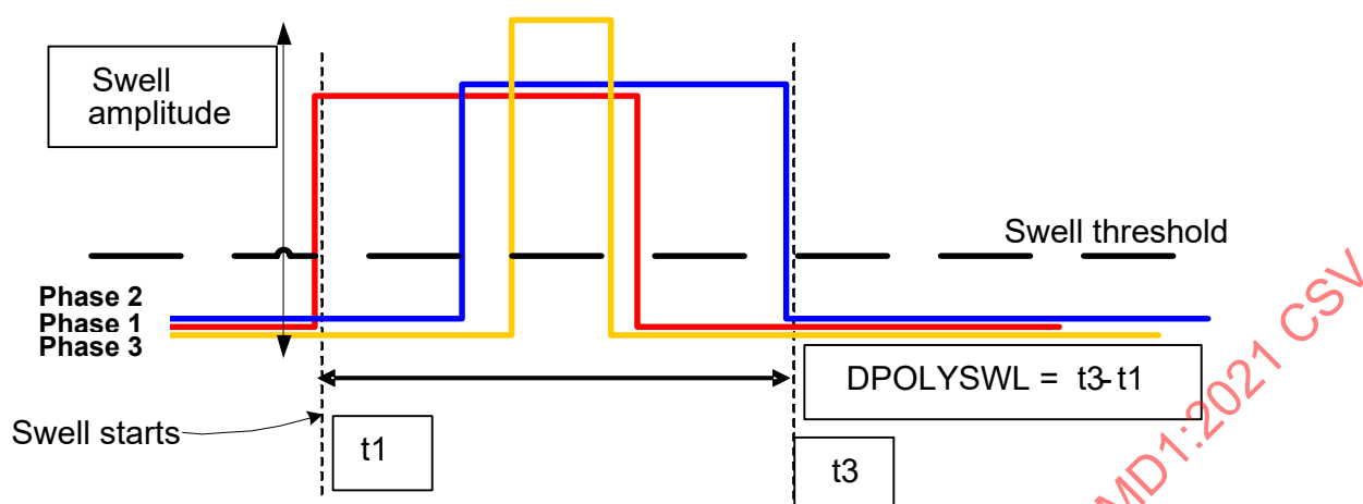
Figure 43 – Detail 1 of waveform for test of polyphase swells
