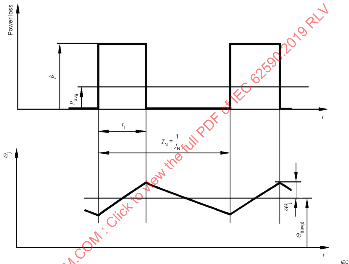
Figure B.2 – Calculation of the virtual junction temperature for continuous load
