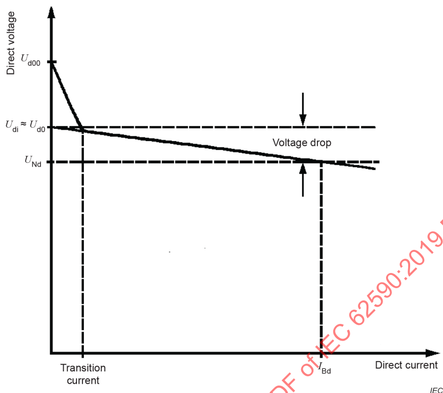
Figure 2 – Voltage drop regulation
