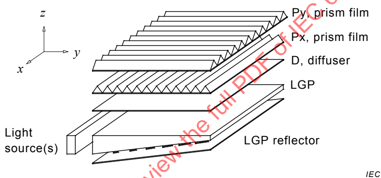
a) Conventional edge-lit backlight unit with arbitrary light sources
