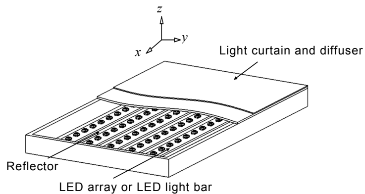
Figure A.3 – Example of a direct-lit backlight unit
