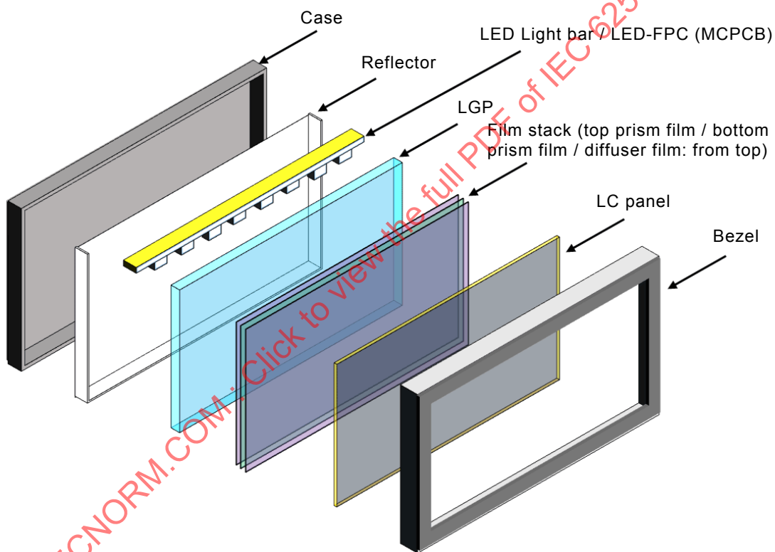
Figure A.4 – Visual definition of the terms related to passive optical components such as bezel and case
