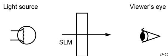
Figure A.1 – Backlighting concept for transmissive and transreflective LCDs
