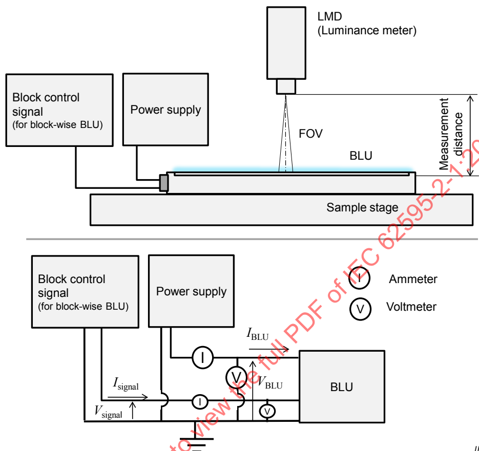
Figure 1 – Example of measuring setup for LED BLU
