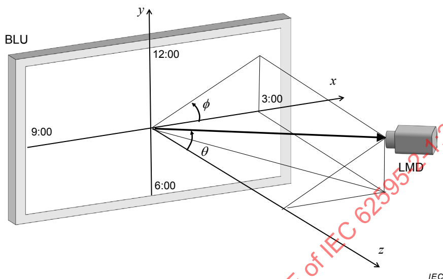
Figure 3 – Definition of zenith angle \theta and azimuth angle \phi
