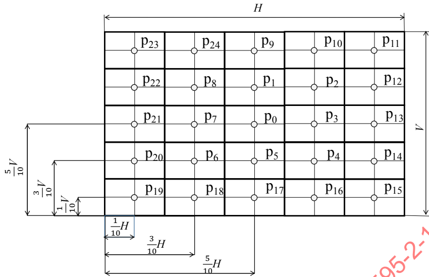
Figure 4 – Examples of measurement point layout
