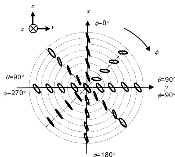
Figure 5 – Example of light polarizing characteristics of an FLU in inverted state
