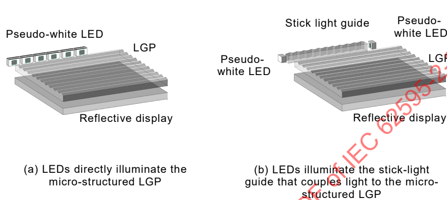
Figure A.1 – Direct edge-lit FLU and indirect edge-lit FLU
