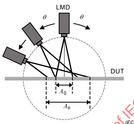
Figure C.1 –Standard goniometric system
