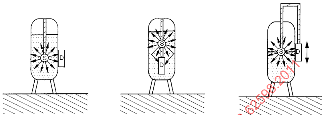
Gauge with the radioactive source inside the material container
