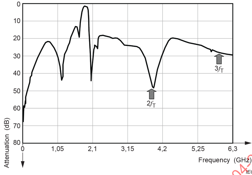
c) Amplitude response of the duplexer from TX port to antenna port (DC to 6 GHz)
