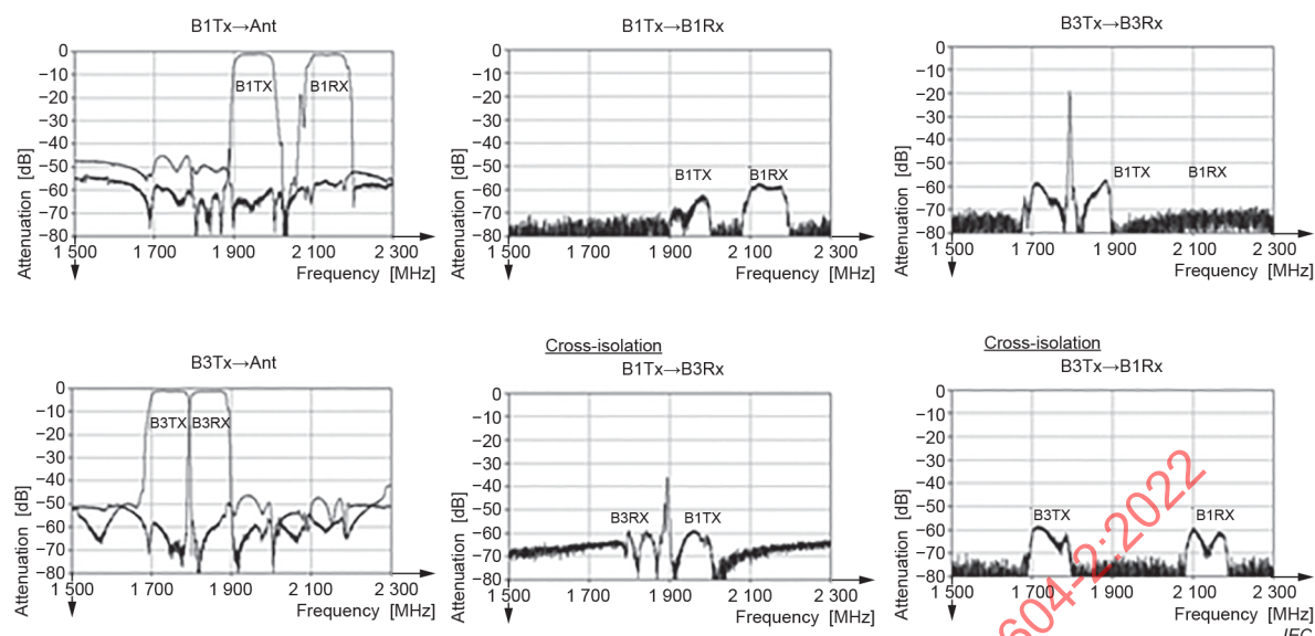
Figure 19 – Frequency characteristics of SAW Band 1 + Band 3 multiplexer for LTE
