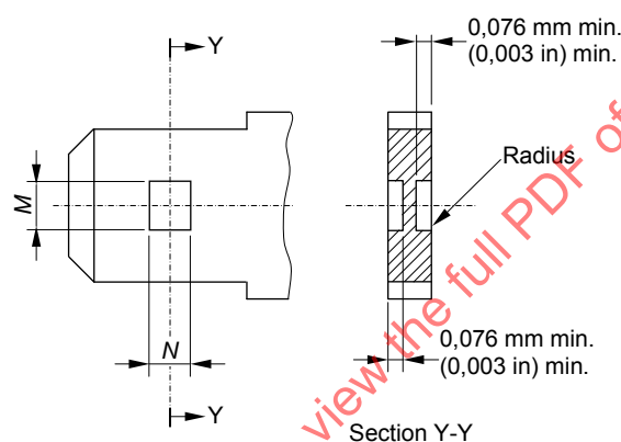
Section Y-Y
