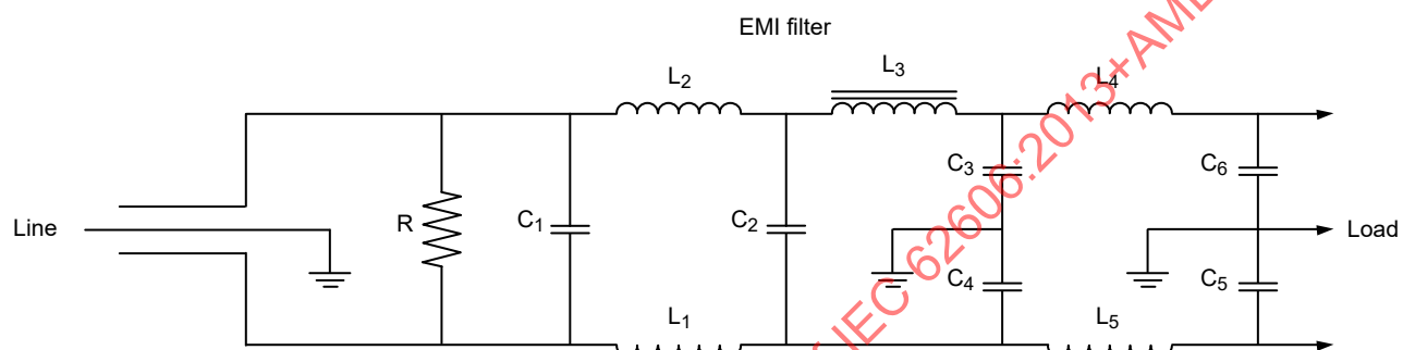
Figure 13 – EMI filter 2 for masking tests
