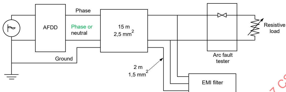
Figure 13 – EMI filter 2 for masking tests
