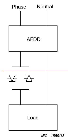
Figure 17 – Controlled current test circuit Void
