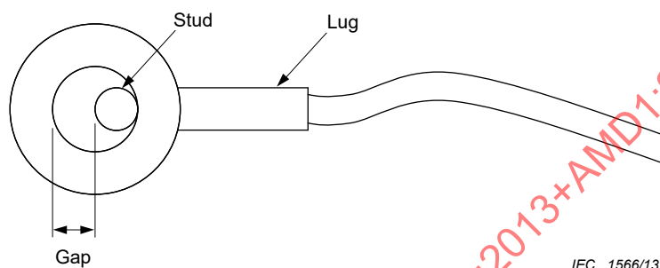
Figure F.1 – Gap Measurement
