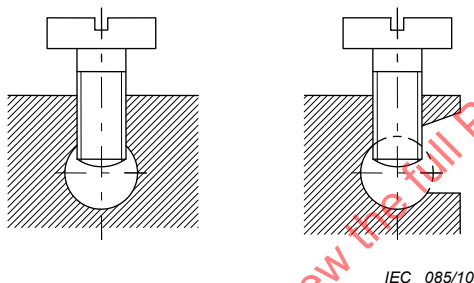
Figure IB.1b – Bornes sans plaquette
