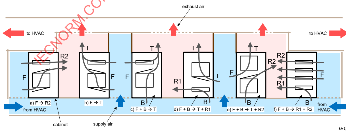
Figure 8 – Example of cabinet airflows in an aisle containment server room
