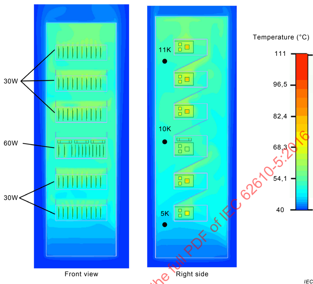
Figure A.3 – Thermal simulation example – Type B
