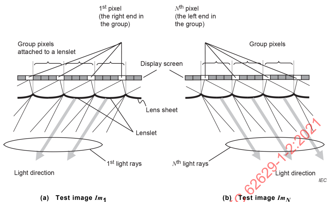
Figure A.2 – Structure of multi-view display 2
