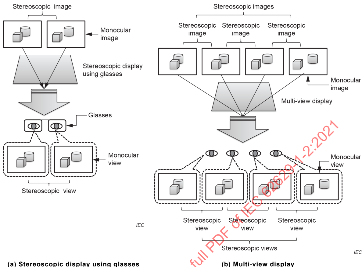
Figure A.3 – Stereoscopic images and stereoscopic views
