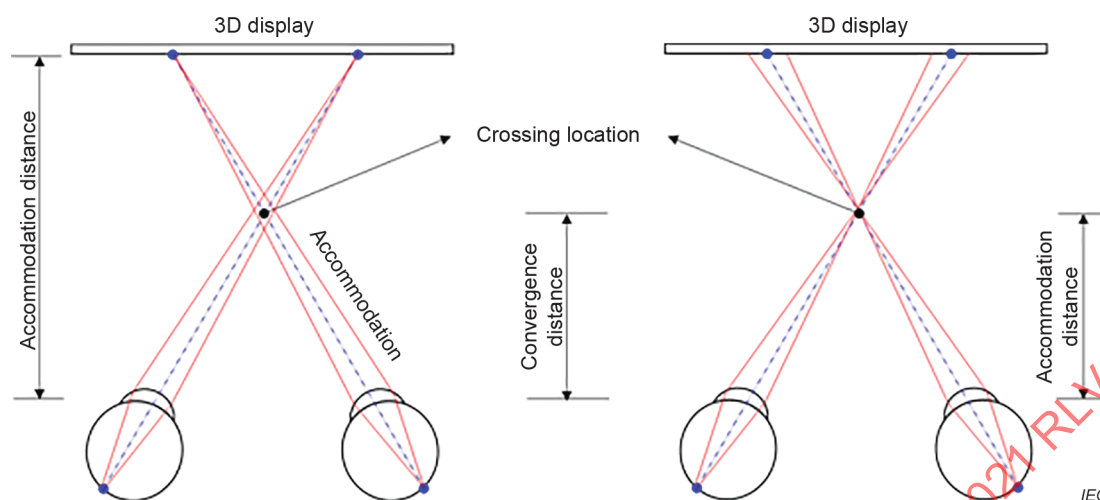
Figure C.2 – Vergence-accommodation conflict
