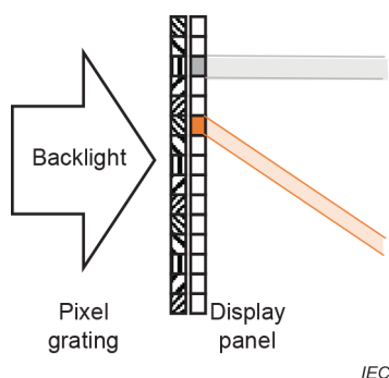
(c) Display panel + grating array
