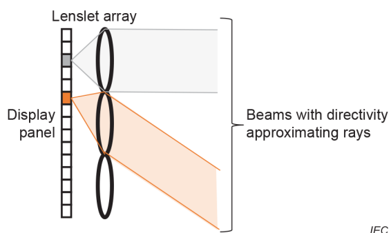
(a) Display panel + lenslet array
