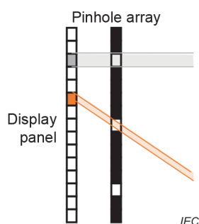
(b) Display panel + pinhole array
