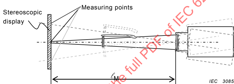
Figure 13 – Layout of glasses for larger aperture LMD for multi-point measurement with head-still condition
