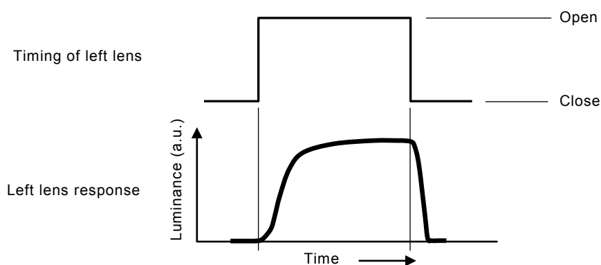
Figure 26 – Example of observed response waveform
