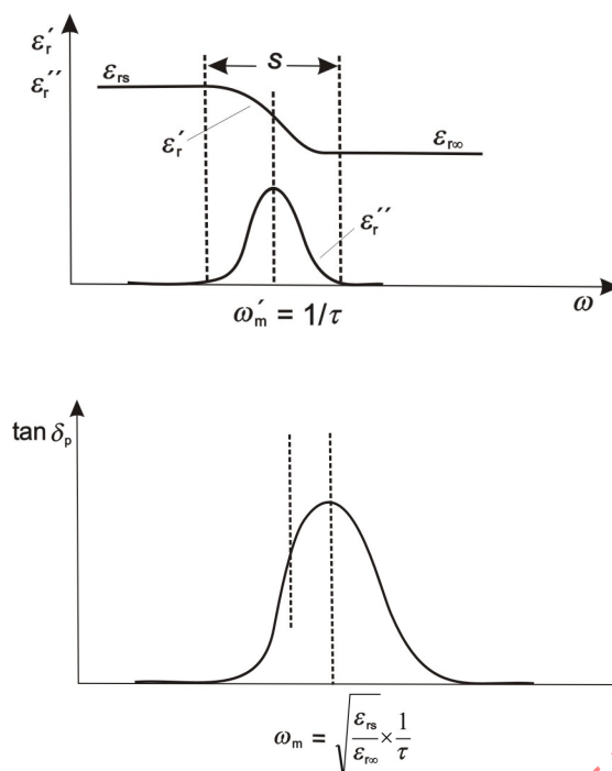
Figure 3 – Influence of frequency \omega = 2\pi f on permittivity and dielectric dissipation factor \tan \delta
