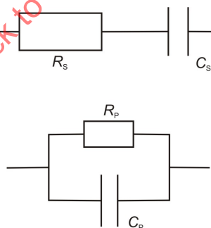
Figure 2 – Equivalent circuit diagrams
