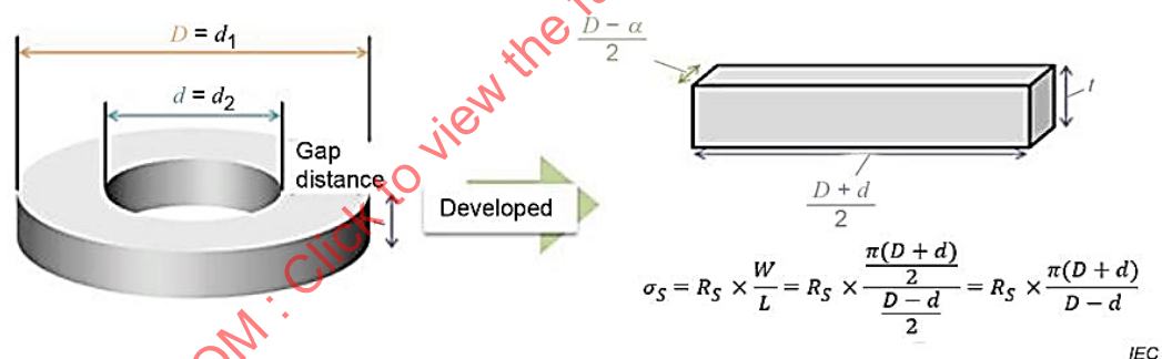
Figure B.1 – Surface resistivity equations for the used electrodes
