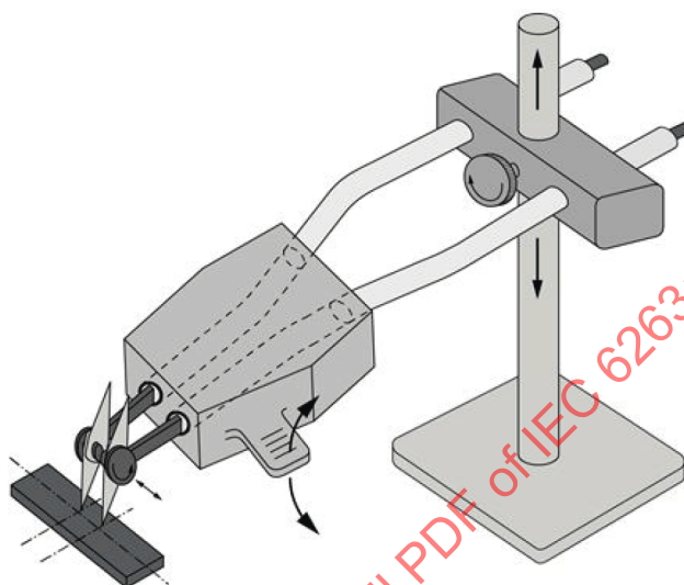
Figure 2 – Collector electrode for electrode arrangement B Electrode arrangement B (example)
