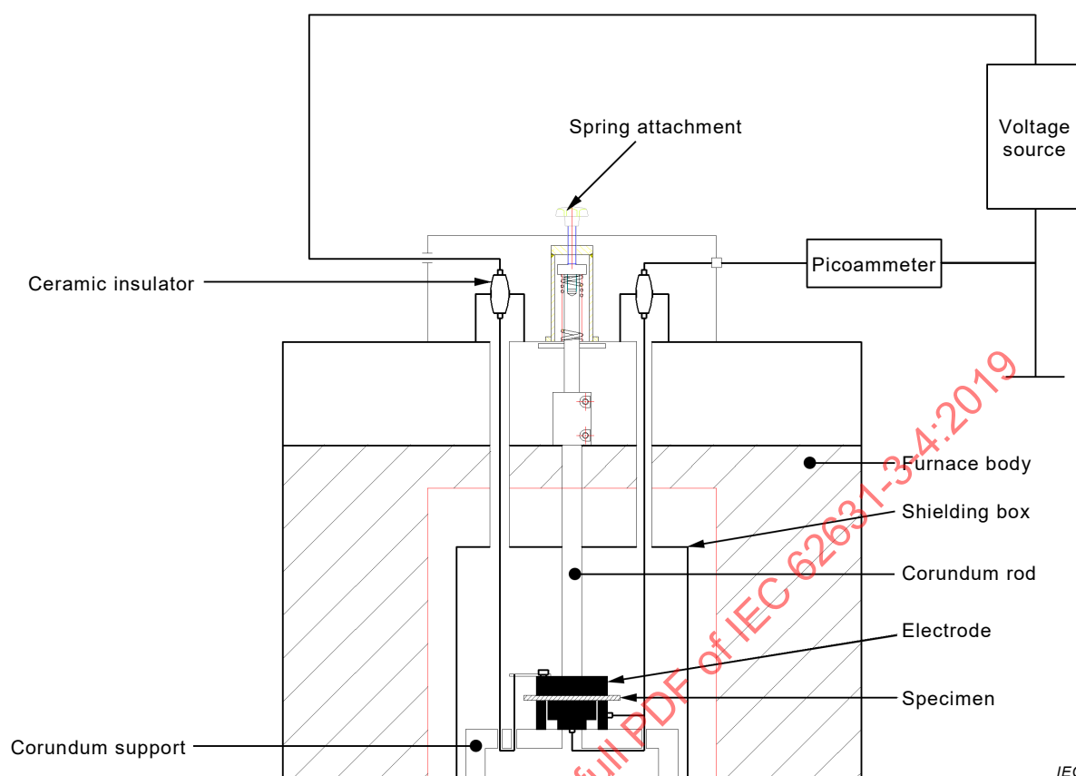
Figure A.2 – Structure diagram of test apparatus
