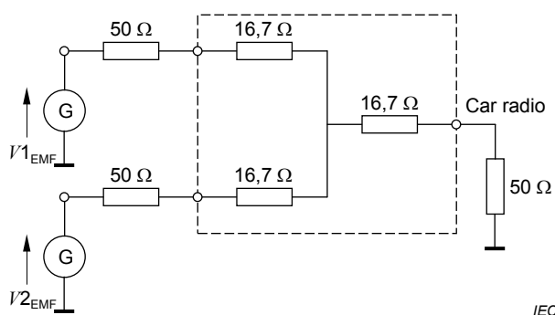
Figure 1 – Coupling circuit
