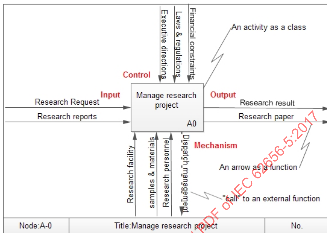
Figure 6 – Sample activity drawing in IDEF0 and ICOM
