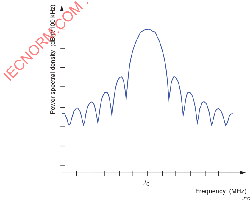
Figure 14 – Power spectral density of an IEEE 802.15.4 system
