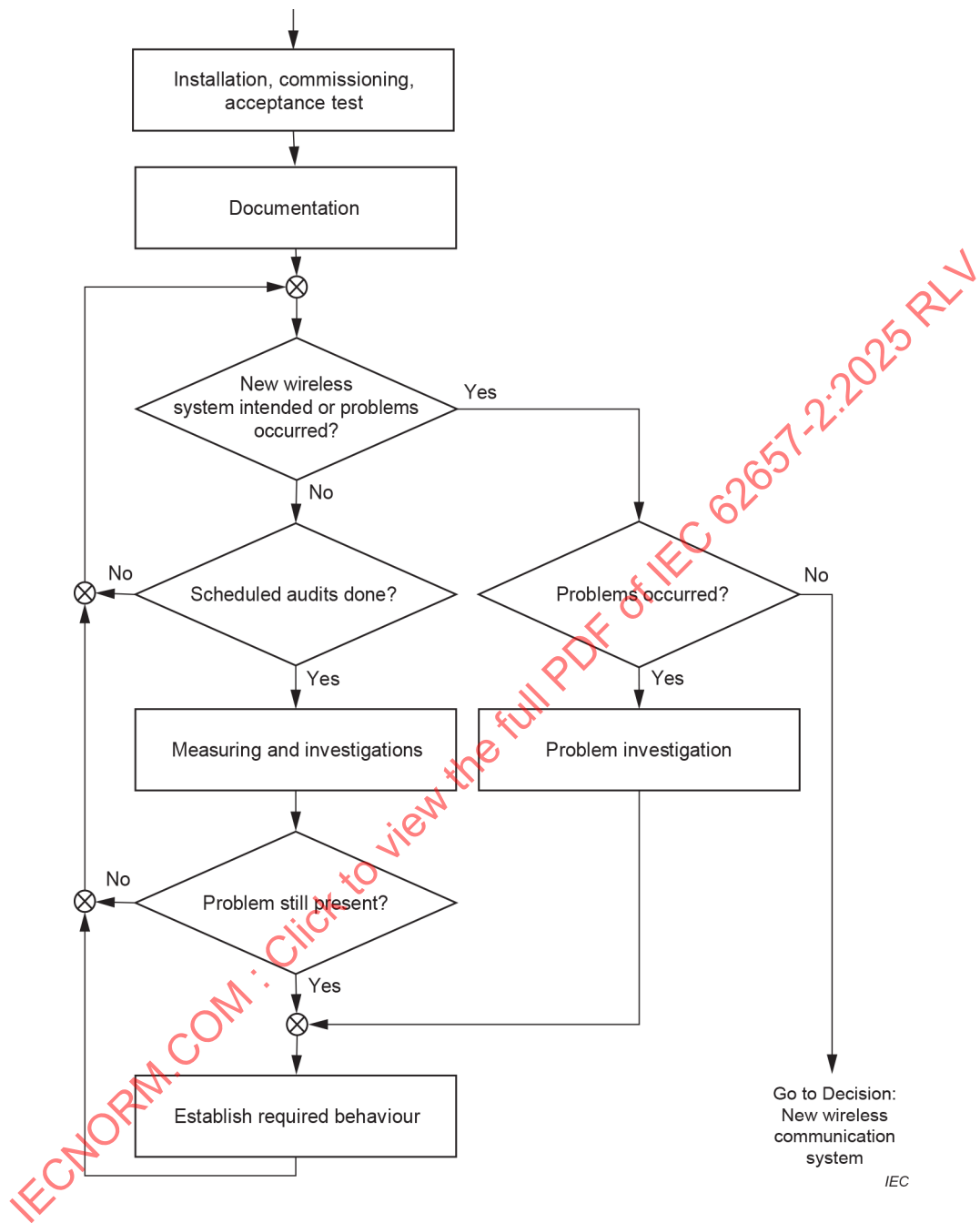
Figure 30 – Implementation and operation of a wireless system in the coexistence management process
