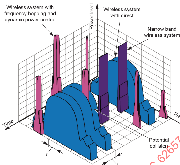
Figure 4 – Separation of wireless systems according to frequency and time
