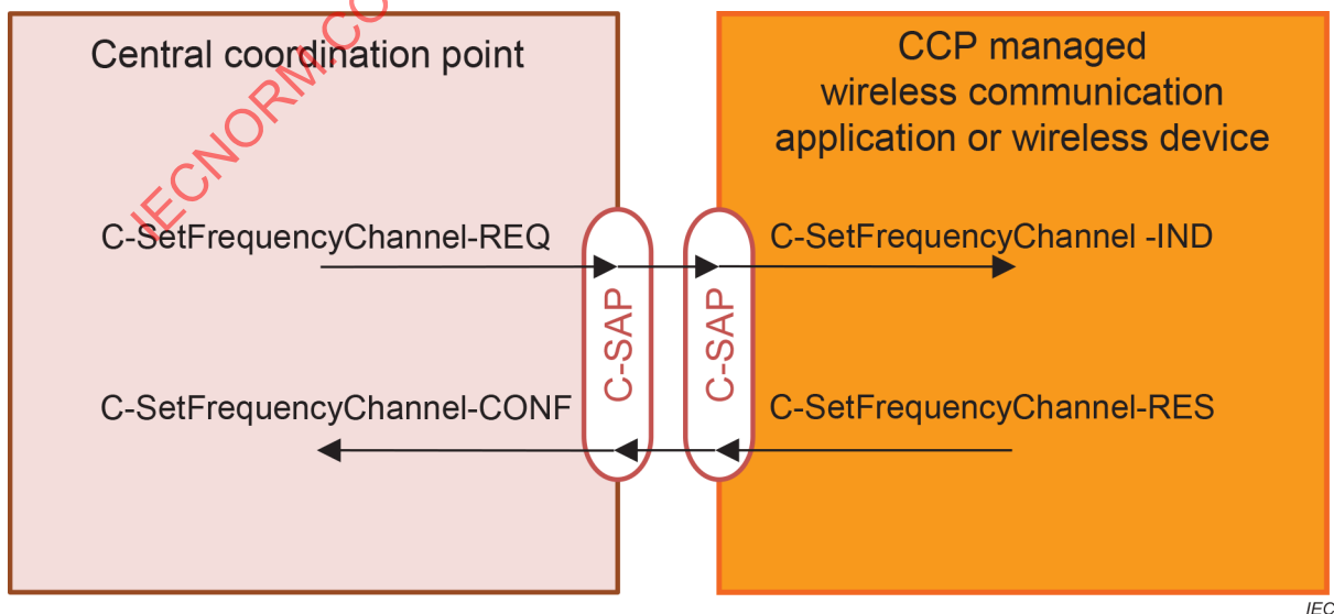
Figure 36 – Primitive flow of SetFrequencyChannel service
