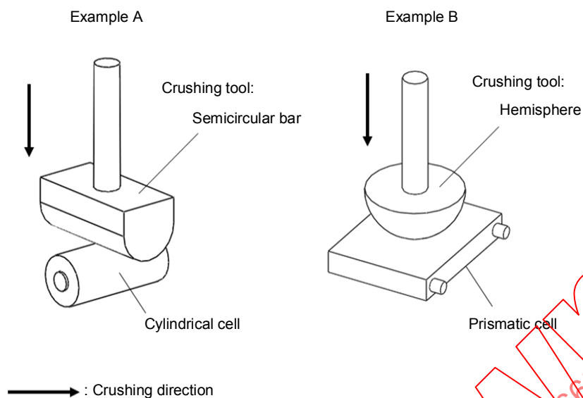
Figure 3 – Example of crush test
