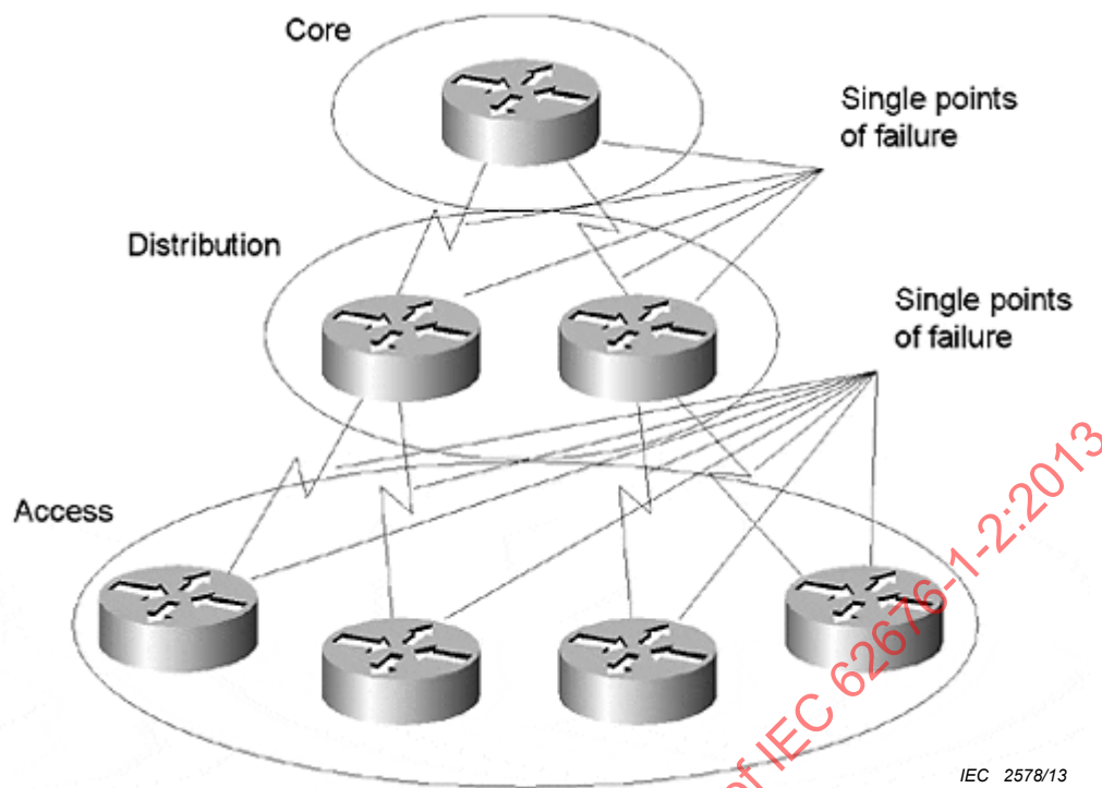
Figure 6 – Hierarchical network
