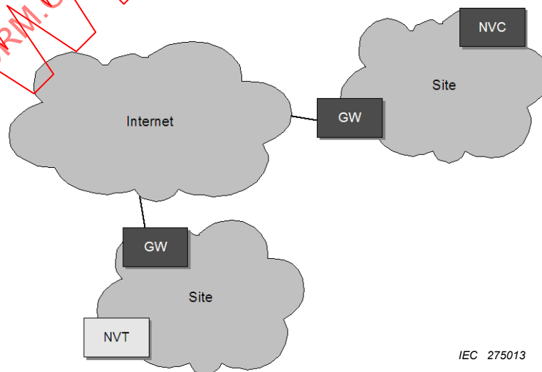
Figure 10 – A device, for example a NVT, in an administrative domain (private) and the client (NVC) in another administrative domain (private)
