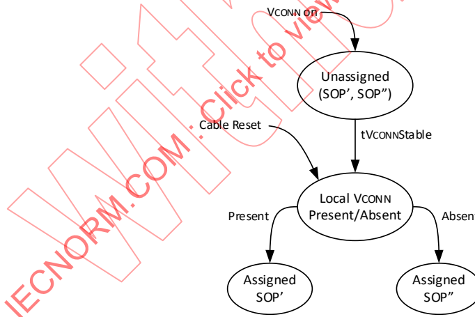
Figure 5-6 Managed Active Cable Plug SOP' and SOP'' Assignment
