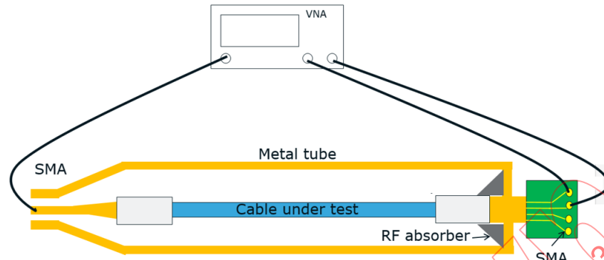
Figure 3-55 Cable Assembly Shielding Effectiveness Testing
