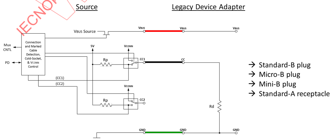
Figure 4-26 Source to Legacy Device Port Functional Model
