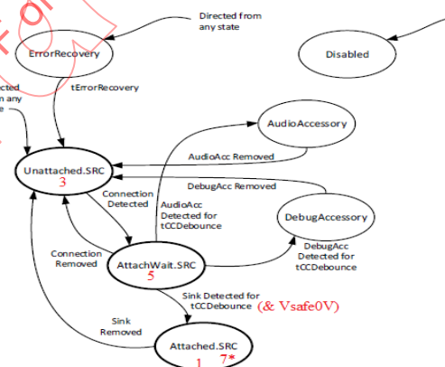
Figure 4-12 Connection State Diagram: Source
