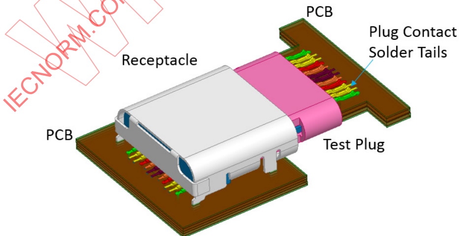
Figure 3-48 Illustration of USB Type-C Mated Connector
