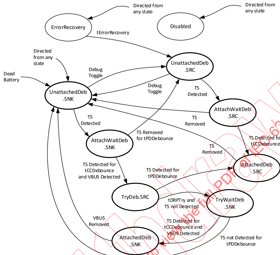
Figure 5-8 Connection State Diagram: DTS DRP
