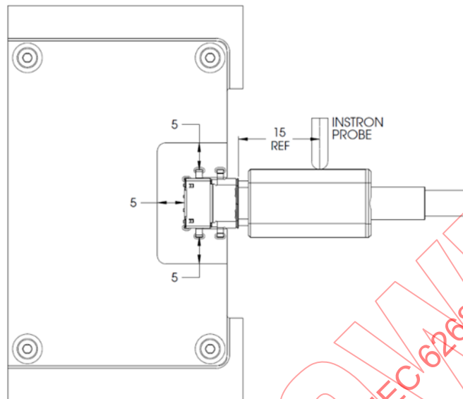
Figure 3-60 Example of 4-Axis Continuity Test Fixture, cont.
