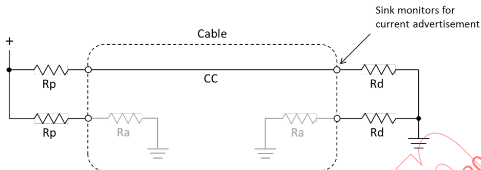
Figure 4-30 Sink Monitoring for Current in Pull-Up/Pull-Down CC Model
