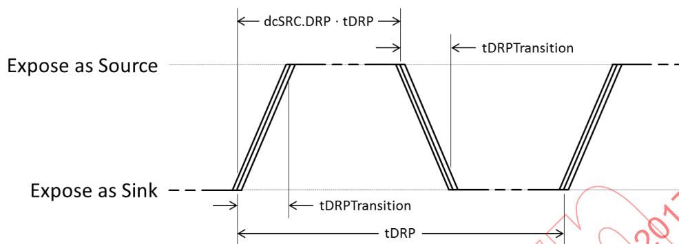
Figure 4-39 DRP Timing
