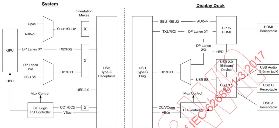
Figure 5-5 USB DisplayPort Dock Example
