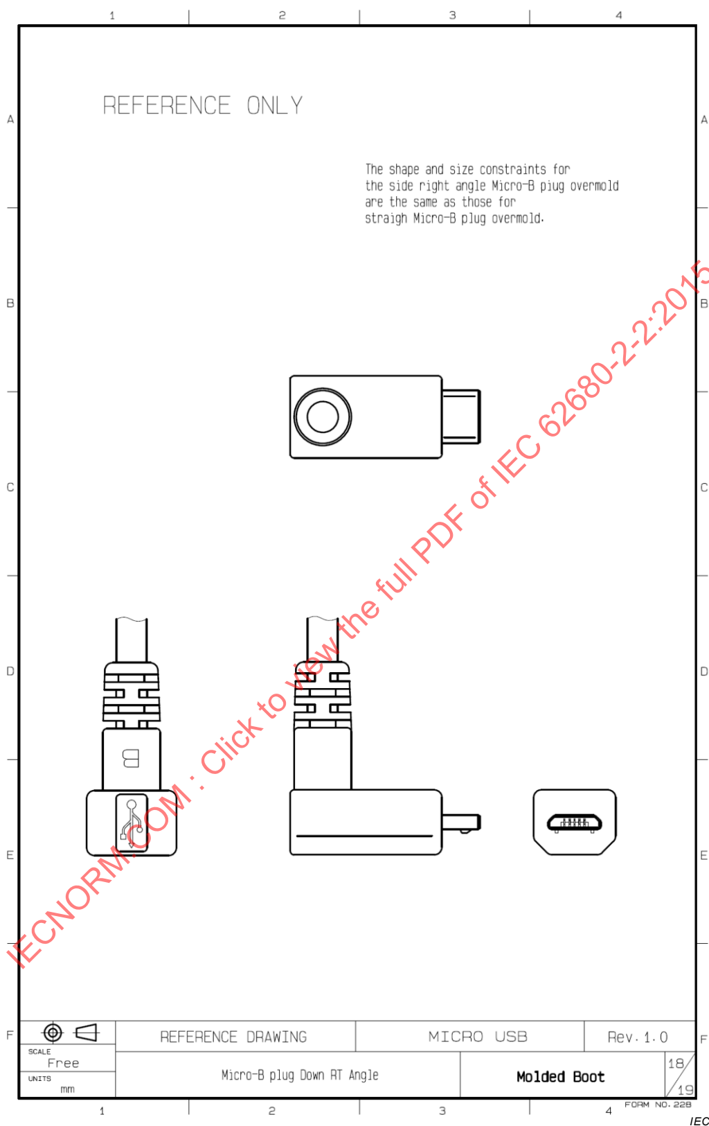
Figure 4-18 – Micro-B Plug, Down Right Angle
