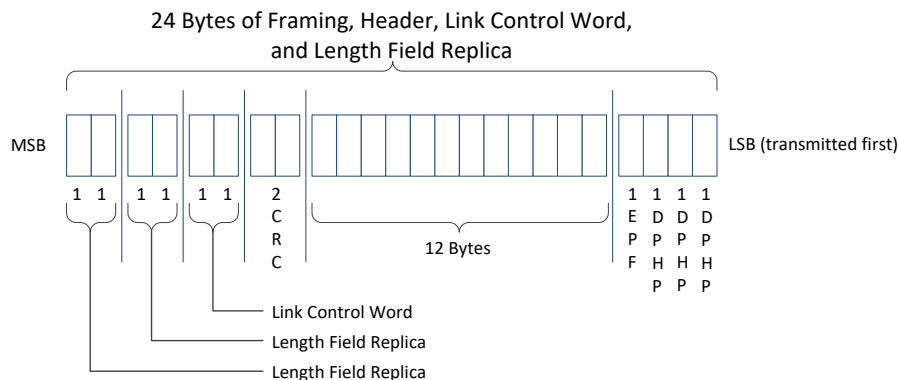
Figure 7-4 – SuperSpeedPlus DPH Format
