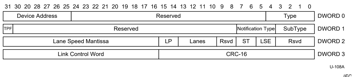
Figure 8-27 – Sublink Speed Device Notification
