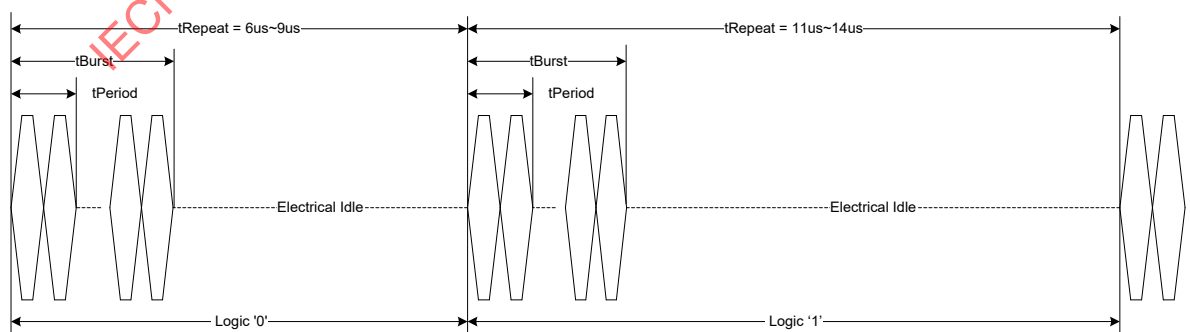
Figure 6-32 – Example of Binary Representation based on Polling.LFPS
