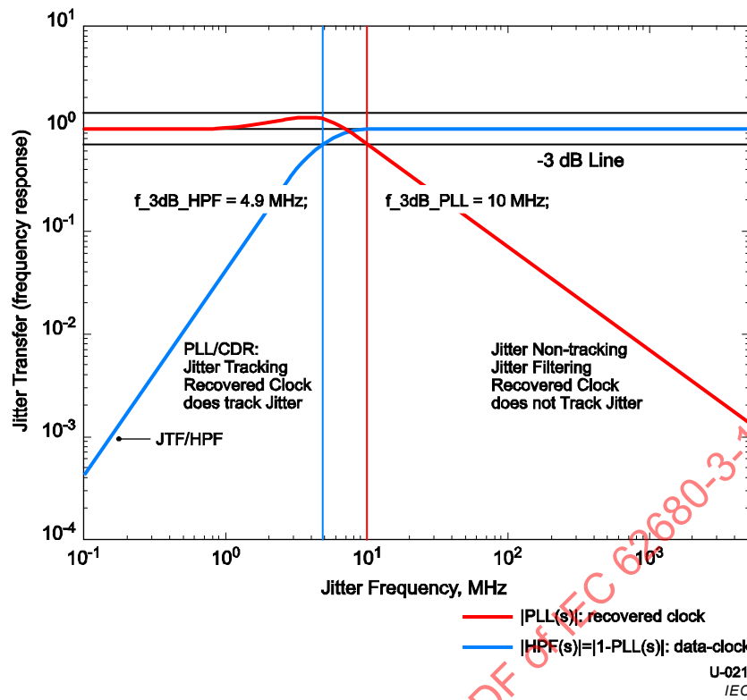
Figure 6-13 – “Golden PLL” and Jitter Transfer Functions for Gen 1 Operation
