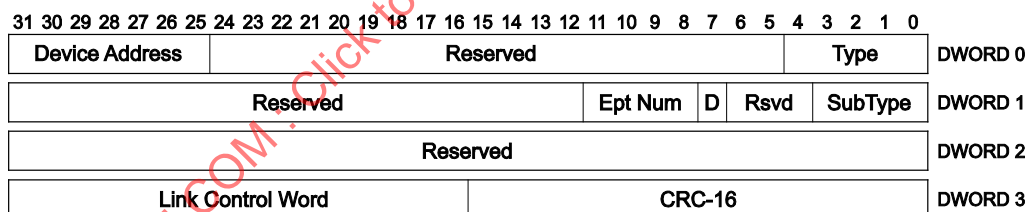
Figure 8-22 – STALL Transaction Packet
