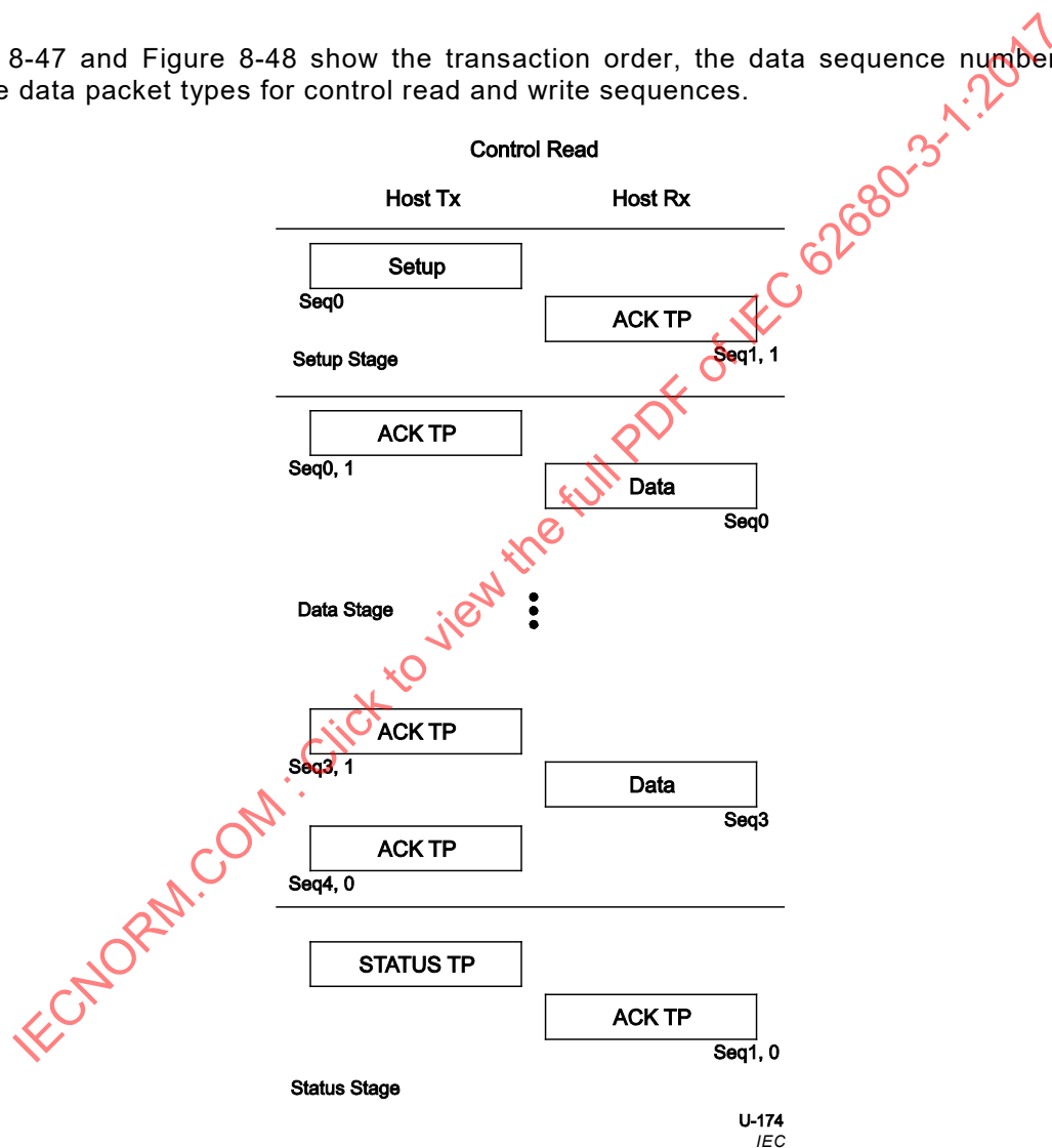
Figure 8-47 – Control Read Sequence
