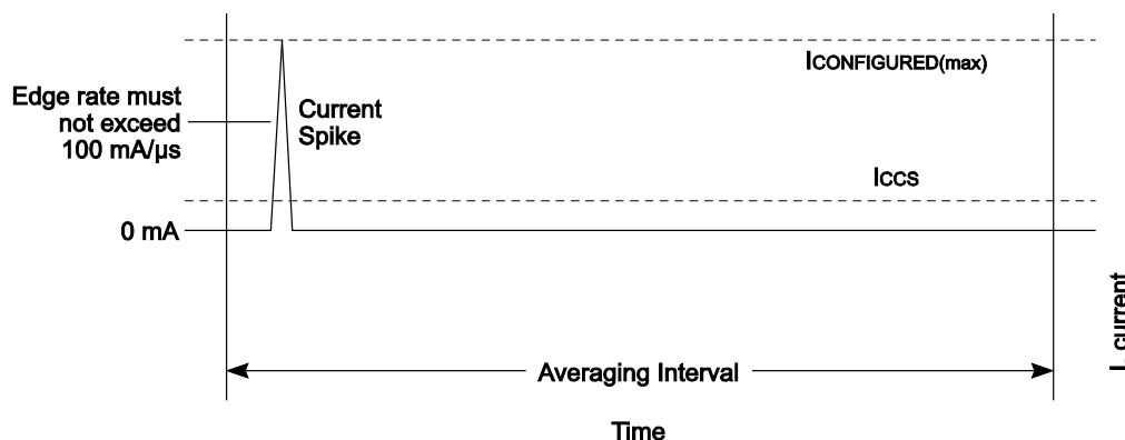
Figure 11-7 – Typical Suspend Current Averaging Profile
