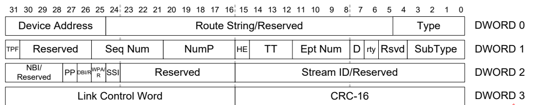
Figure 8-18 – ACK Transaction Packet
