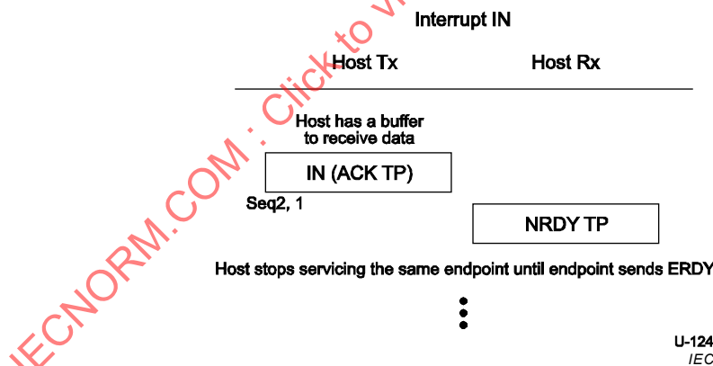
Figure 8-50 – Host Stops Servicing Interrupt IN Transaction Once NRDY is Received
