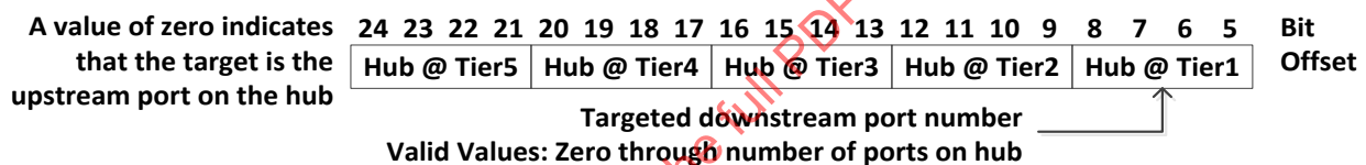
Figure 8-32 – Route String Detail
