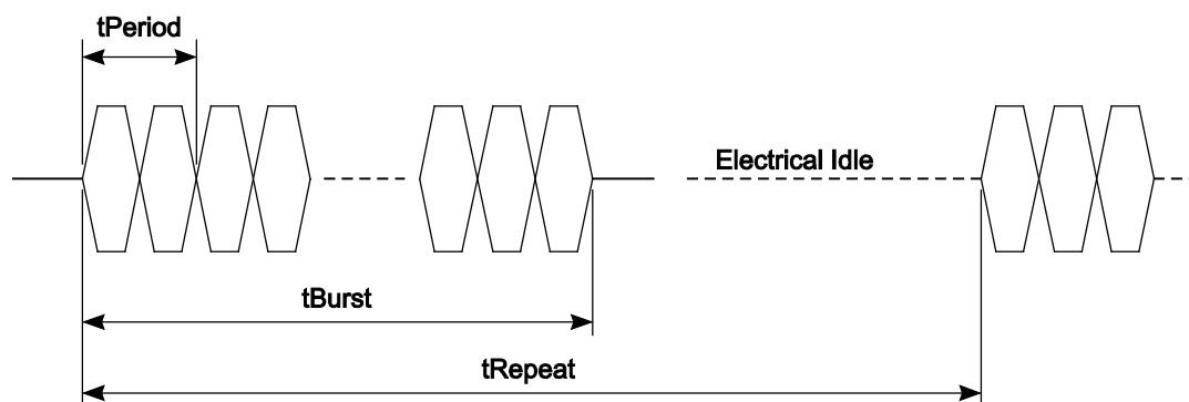
Figure 6-29 – LFPS Signaling
