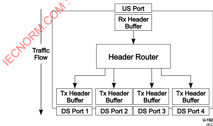
Figure 10-15 – Example SS Hub Header Packet Buffer Architecture – Downstream Traffic
