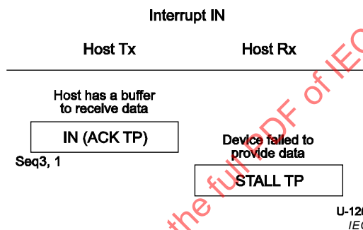
Figure 8-52 – Endpoint Sends STALL TP
