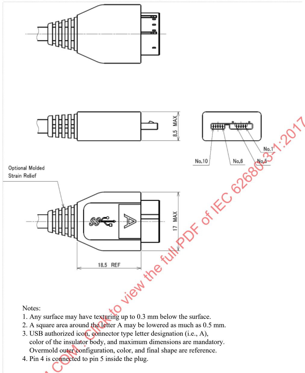
Figure 5-18 – USB 3.1 Micro-A Cable Overmold Dimensions
