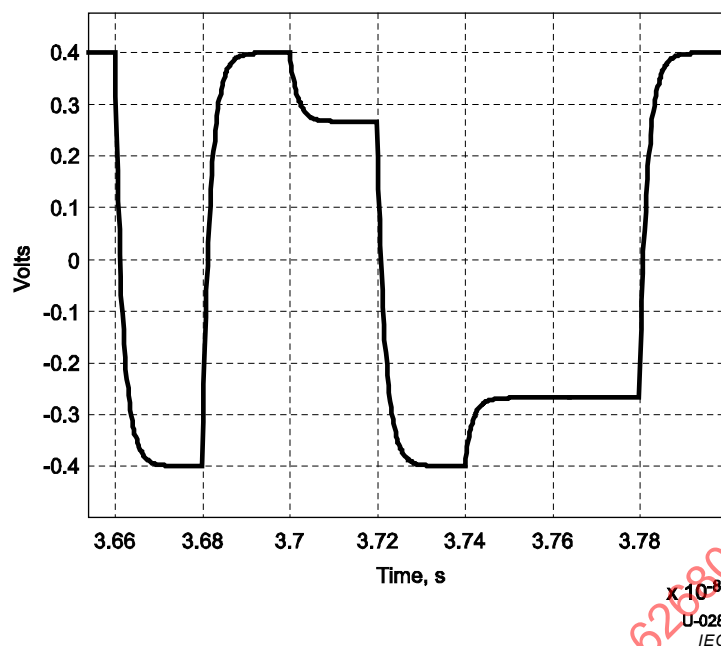
Figure 6-20 – De-Emphasis Waveform
