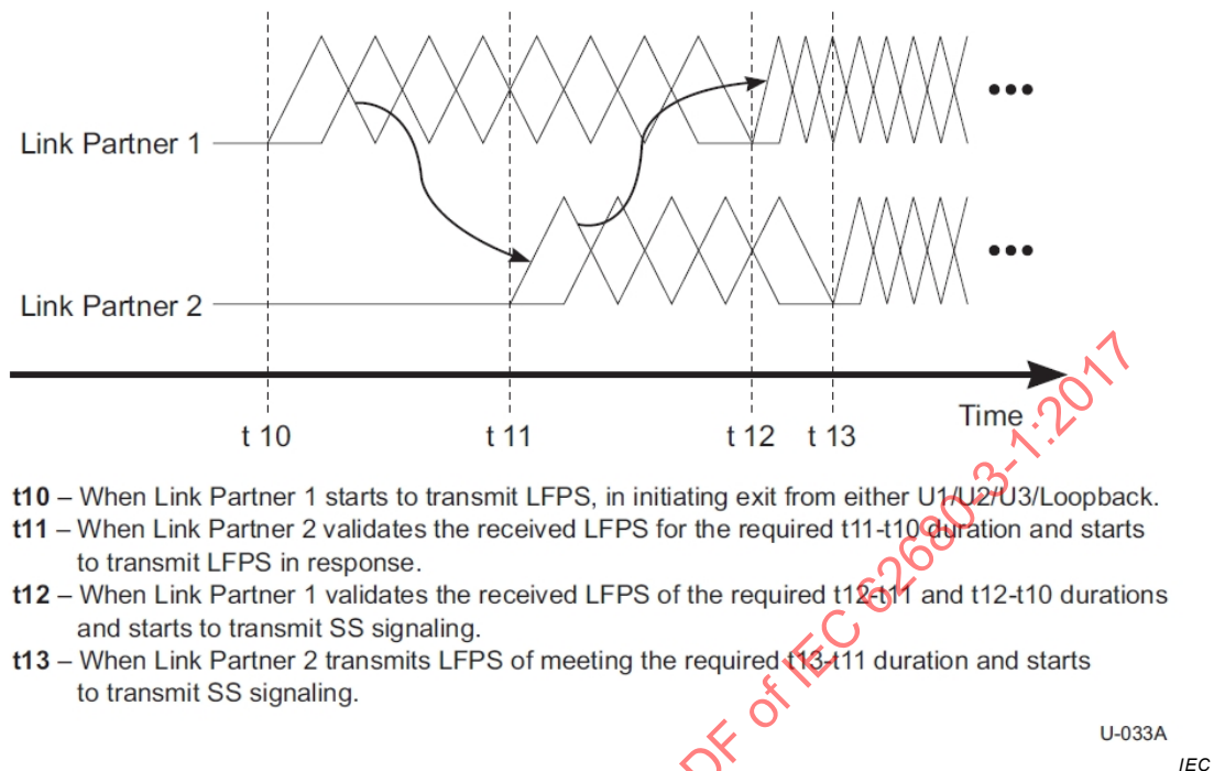
Figure 6-30 – U1 Exit, U2 Exit, and U3 Wakeup LFPS Handshake Timing Diagram
