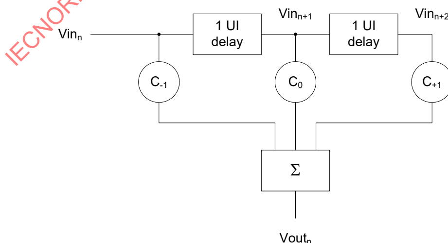
Figure 6-21 – 3-tap Transmit Equalizer Structure
