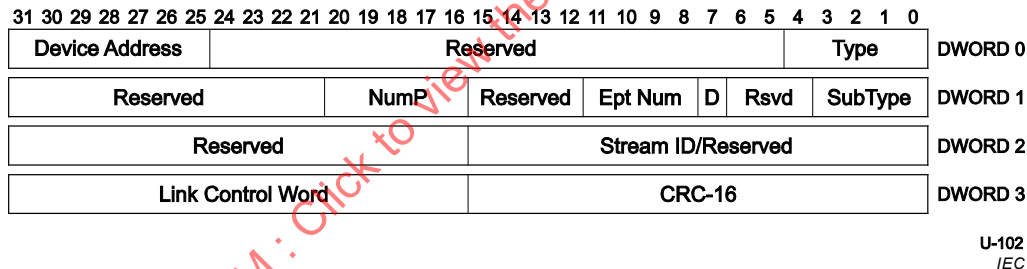
Figure 8-20 – ERDY Transaction Packet
