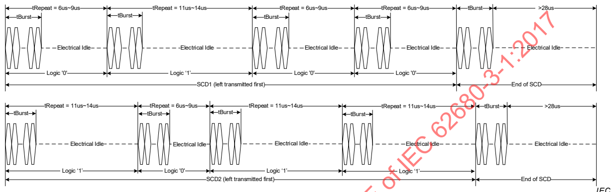
Figure 6-33 – SCD1/SCD2 transmission
