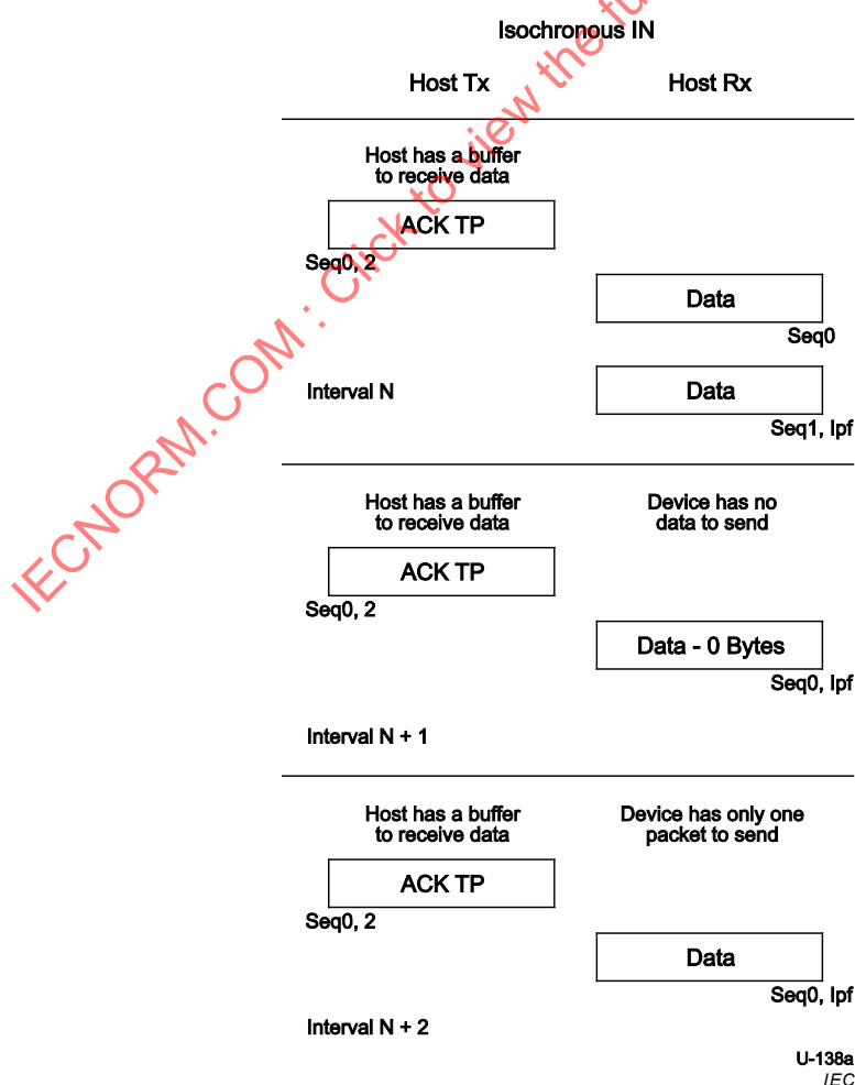
Figure 8-62 – Sample Enhanced SuperSpeed Isochronous IN Transaction
