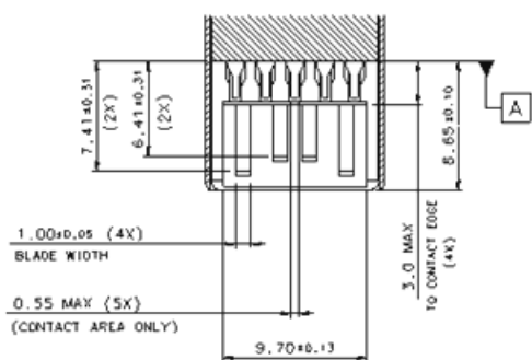
SECTION T-T
