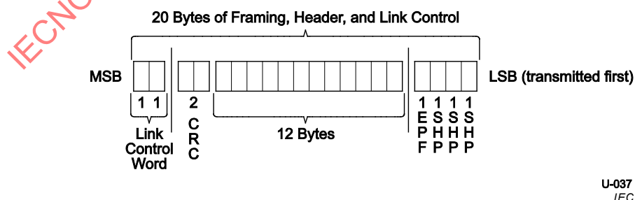
Figure 7-3 – Enhanced SuperSpeed Header Packet with HPSTART, Packet Header, and Link Control Word
