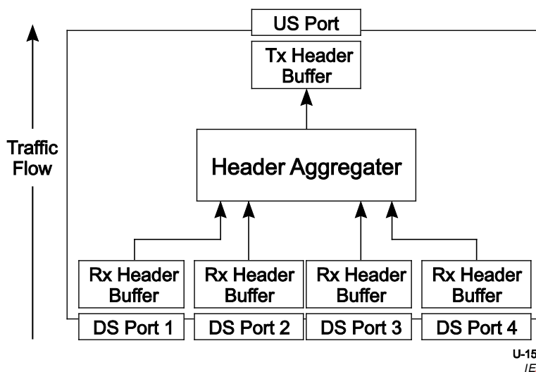
Figure 10-16 – Example SS Hub Header Packet Buffer Architecture – Upstream Traffic
