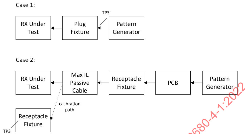
Figure 3-18. Receiver Tolerance Test Topologies
