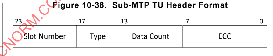
Figure 10-38. Sub-MTP TU Header Format
