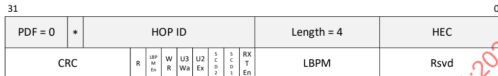
Figure 9-1. LFPS Tunneled Packet Format
