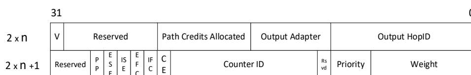
Figure 8-16. Structure of Path Entry ‘n’ in Path Configuration Space at Lane Adapter
