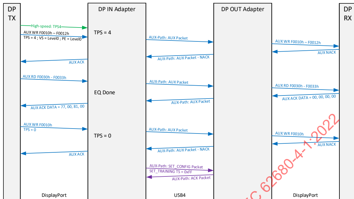
Figure 10-18. DP Link Training – LTTPr – EQ Phase
