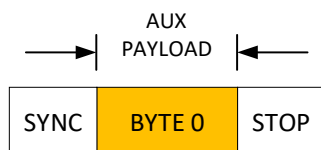
Figure 10-5. AUX Channel Framing
