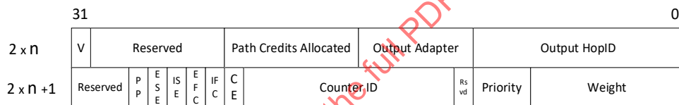
Figure 8-17. Structure of Path Entry ‘n’ in Path Configuration Space of a Protocol Adapter
