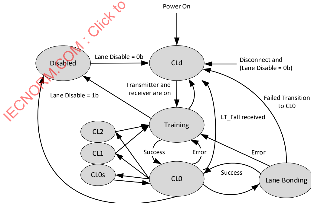
Figure 4-8. The Lane Adapter State Machine
