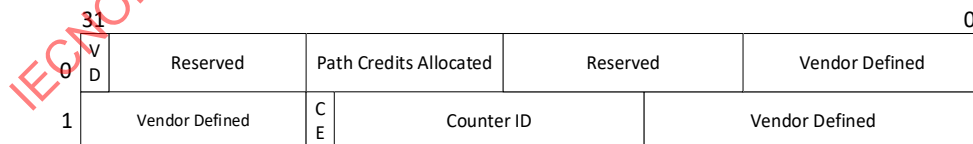
Figure 8-15. Structure of Path 0 Entry Configuration Space
