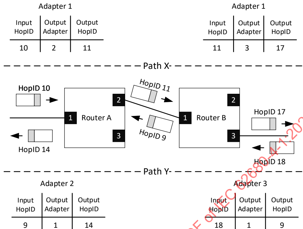
Figure 5-9. Routing Example
