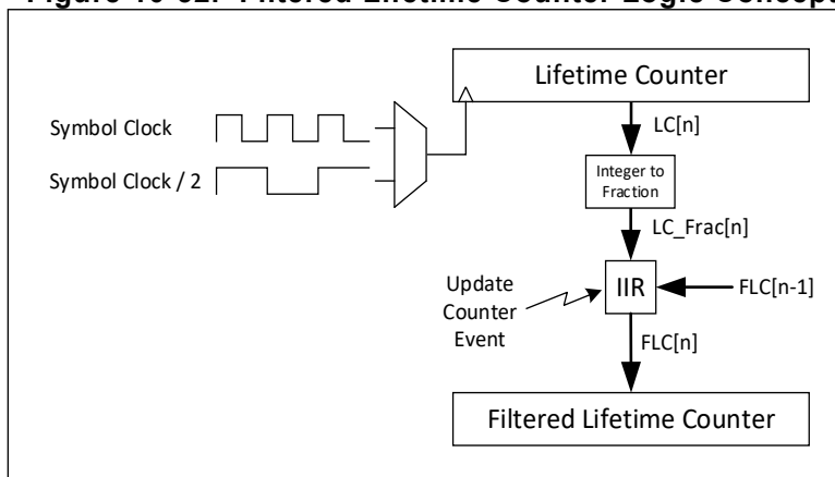
Figure 10-52. Filtered Lifetime Counter Logic Concept
