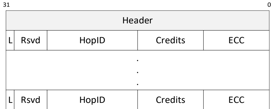
Figure 5-4. Credit Grant Packet Format
