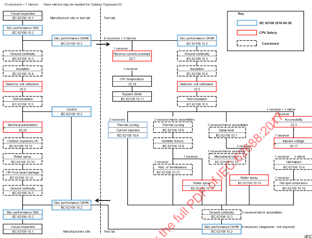
Figure 10 – Combined IEC 62108:2016 and IEC 62688 test plan for CPV assemblies
