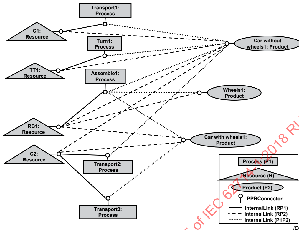
Figure A.31 – Links within the example
