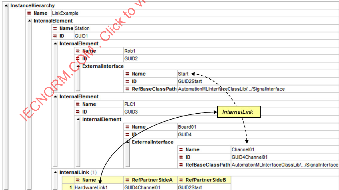
Figure 5 – Example relation between the objects “PLC1” and “Rob1”
