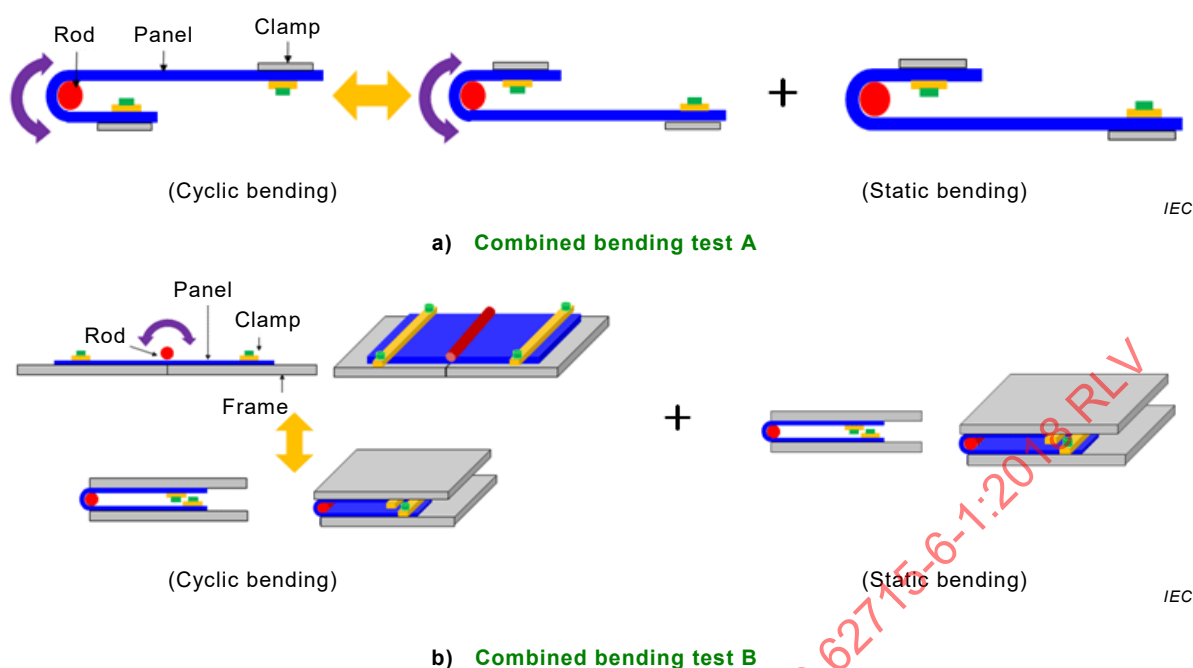
Figure 3 – Apparatus for combined bending tests consisting of the cyclic bending test and static bending test
