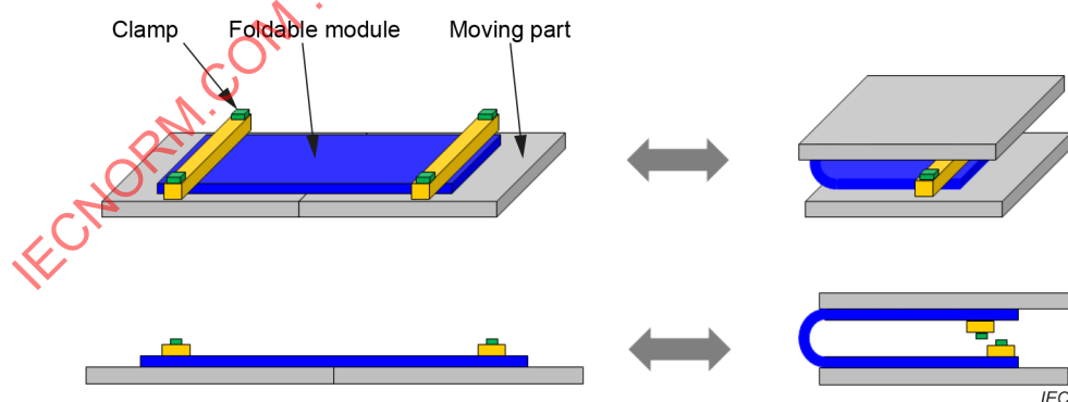
Figure 1 – Example of test apparatus for in-folding type sample
