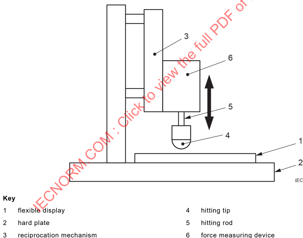
Figure 2 – Example of apparatus for hitting test
