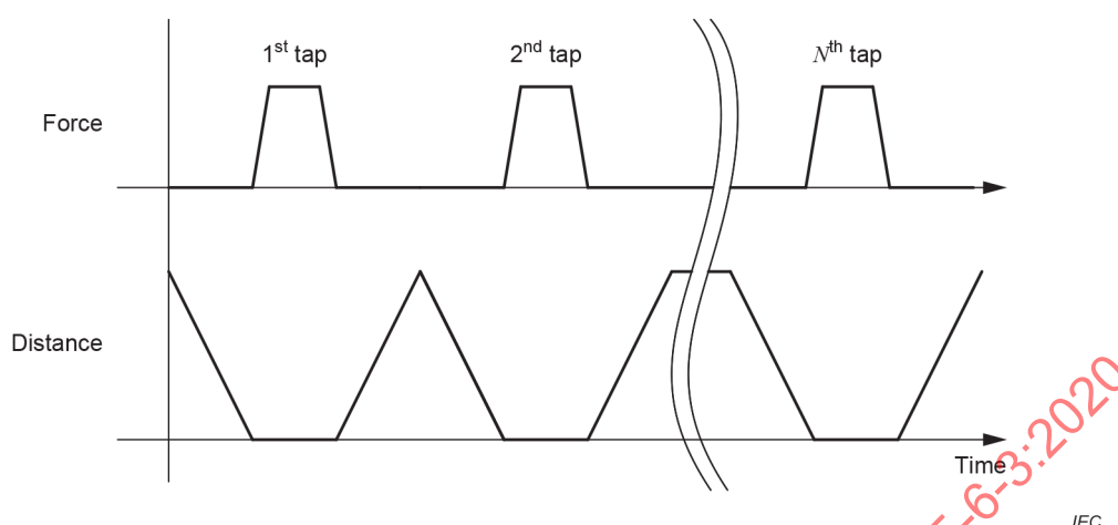
Figure 3 – Example of the tip movement and applied force
