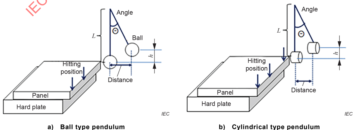
Figure 4 – Apparatus for pendulum side impact test
