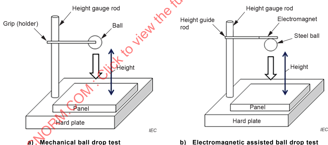
Figure 1 – Apparatus for ball drop test equipment
