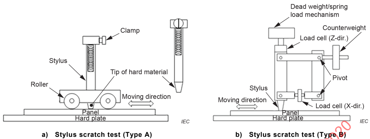
Figure 5 – Apparatuses for stylus scratch test using a stylus holder with different pressures available by modulating the spring load
