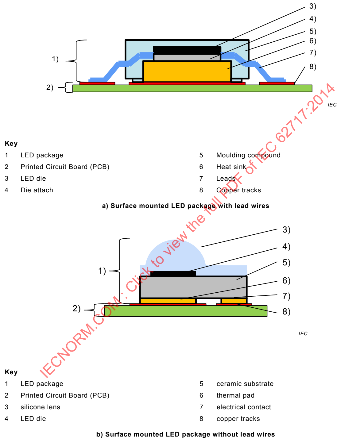
Figure G.2 – Schematic drawings of LED packages
