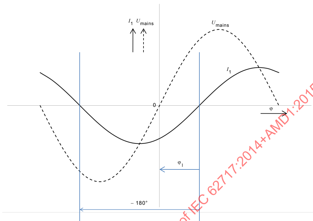
Figure E.2 – Definition of the fundamental current phase shift angle \varphi_1 ( I_1 lags U_{\text{mains}} , \varphi_1 < 0 )
