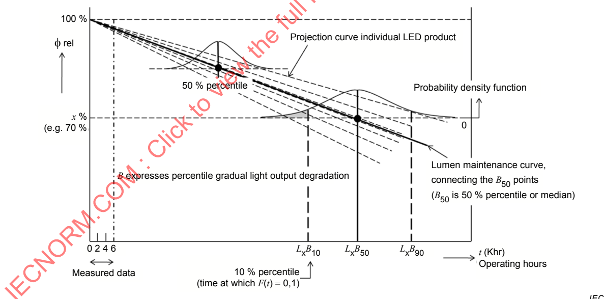
Figure C.2 – Life time specification for gradual light output degradation
