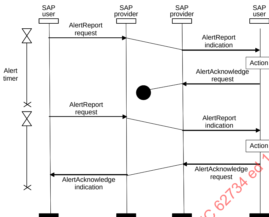
Figure 132 – AlertReport, acknowledgment failure
