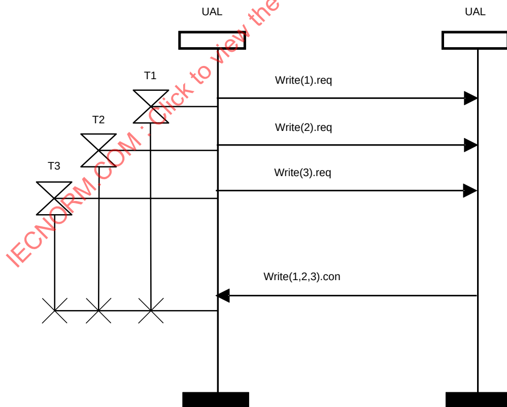
Figure 113 – A successful example of multiple outstanding requests, with response concatenation
