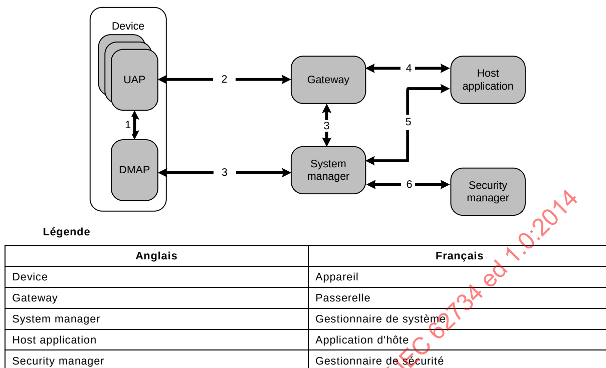
Figure 23 – Architecture de gestion
