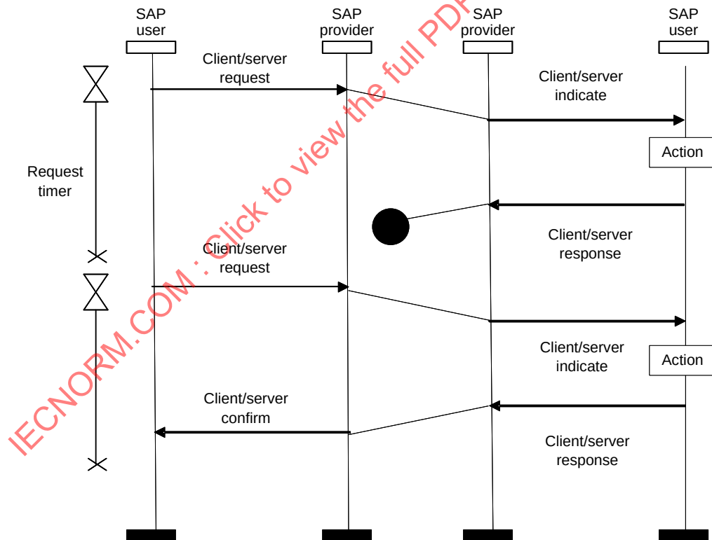
Figure 129 – Client/server model four-part interactions: Response delivery failure
