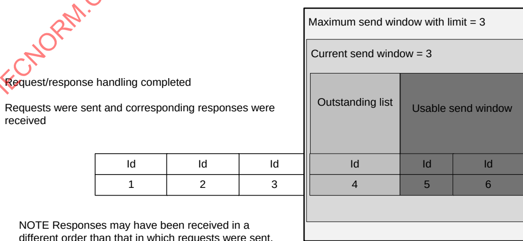
Figure 117 – Send window example 2, with current send window the same size as maximum send window, and non-zero usable send window width
