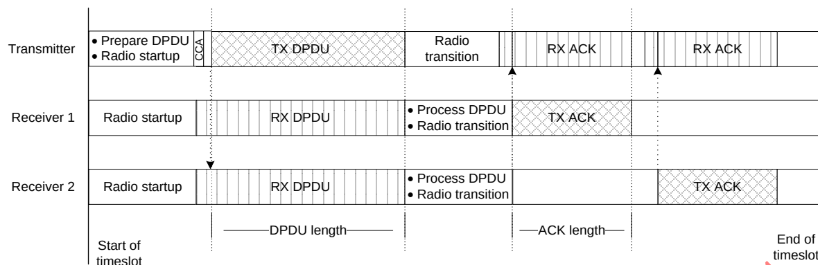
Figure 84 – Duocast transaction
