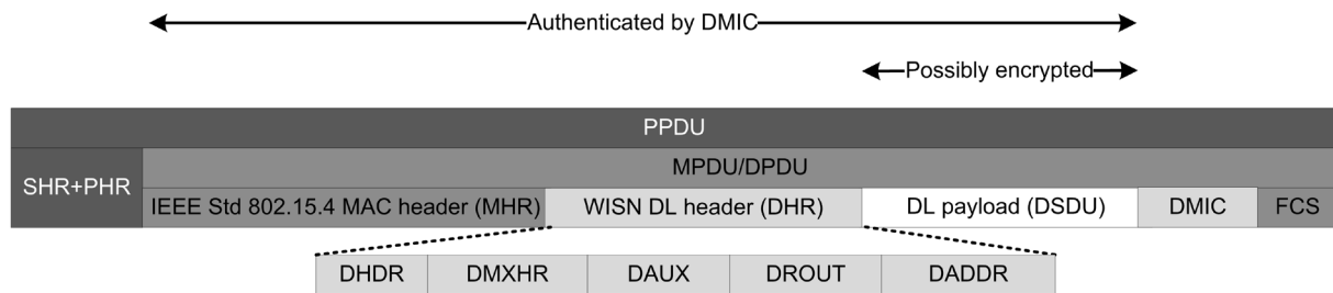
Figure 37 – DPDU structure
