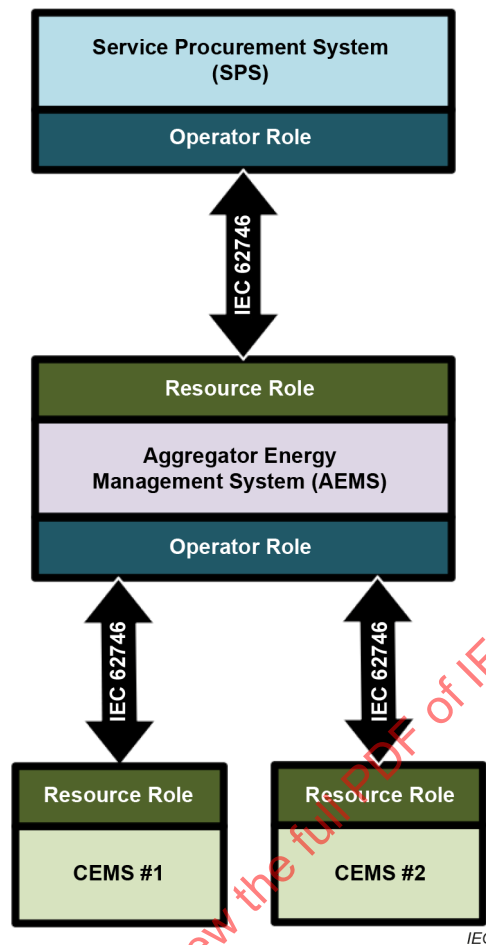
Figure 3 – SPS-AEMS-CEMS communications logical model
