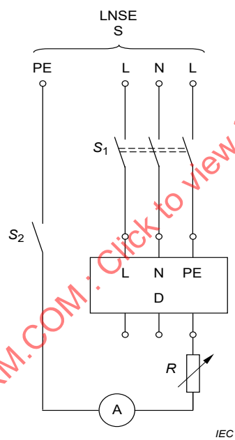
Figure 4c) – Type LNSE
